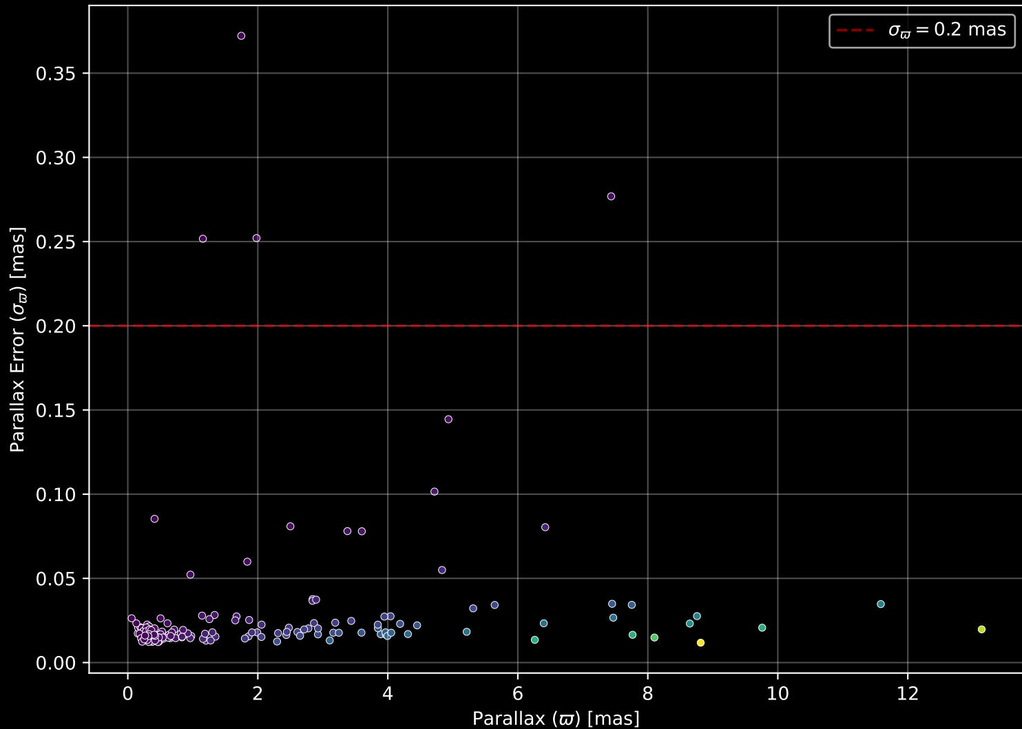
APOGEE DR17 Field: [158+18] Parallax Quality (n= 166)
