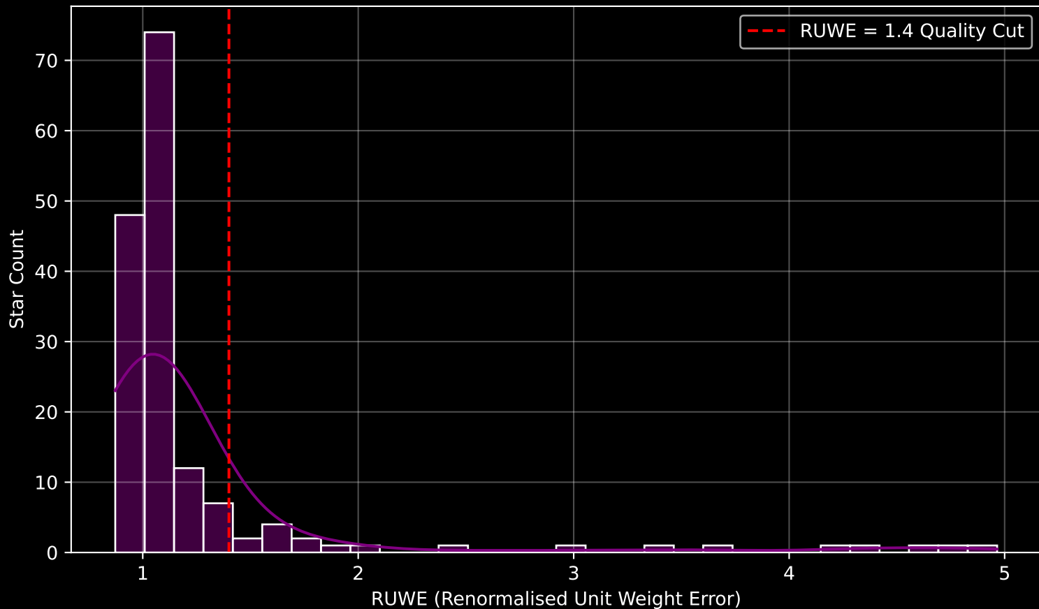
GAPOGEE DR17 Field [158+18] RUWE Distribution (n= 160)
