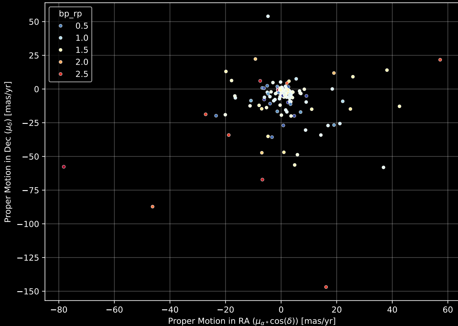
APOGEE DR17 Field: [158+18] Proper Motion Diagram (n= 166)
