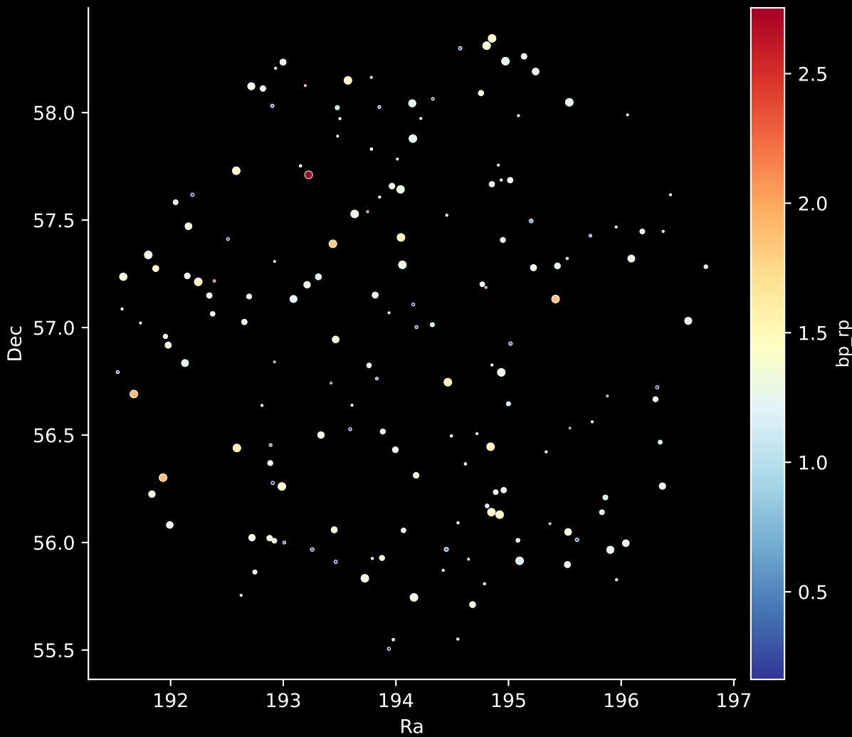
APOGEE DR17 Field: [158+18] Stars: 166
