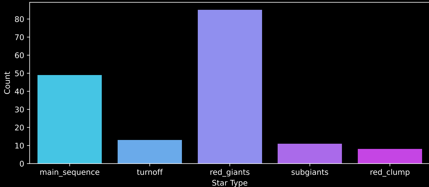
APOGEE DR17 Field: [158+18] Count plot of Star Type
