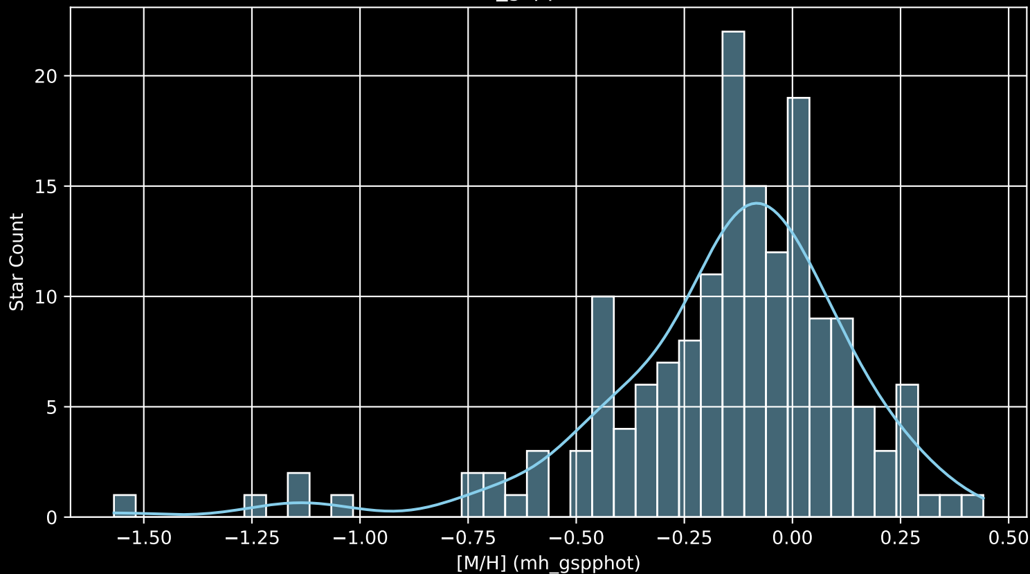
APOGEE DR17 Field: [158+18 [M/H] (mh_gspphot) (n= 165)
